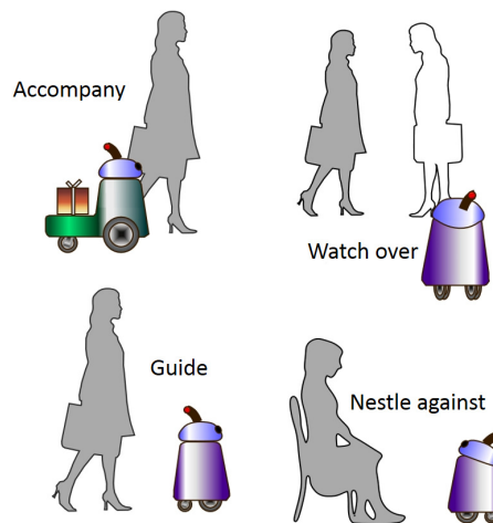
Fig. 1. Adaptive attendance
