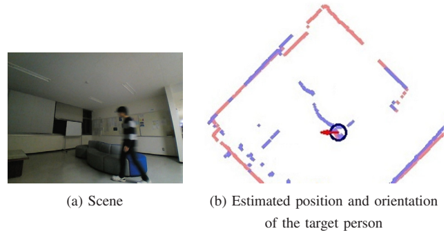
Fig. 3. Person detection with laser range finders
