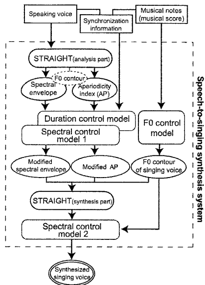
Fig. 1 Block diagram of the proposed singing voice synthesis system.
