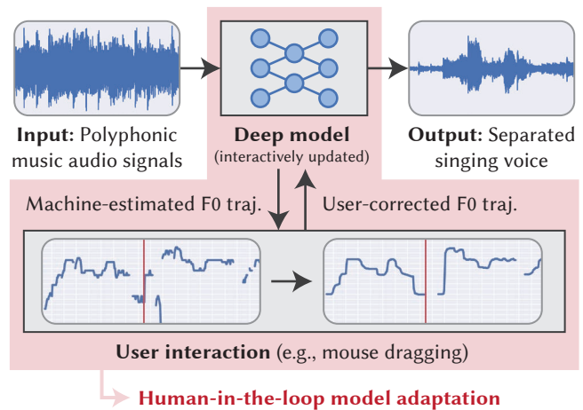
Figure 1: Overview of interactive deep singing-voice separation , where the user can interact with the deep neural network model to fine-tune the quality of the separated singing voice. The user feedback is provided as F0 trajectories, based on which the model is adapted.
