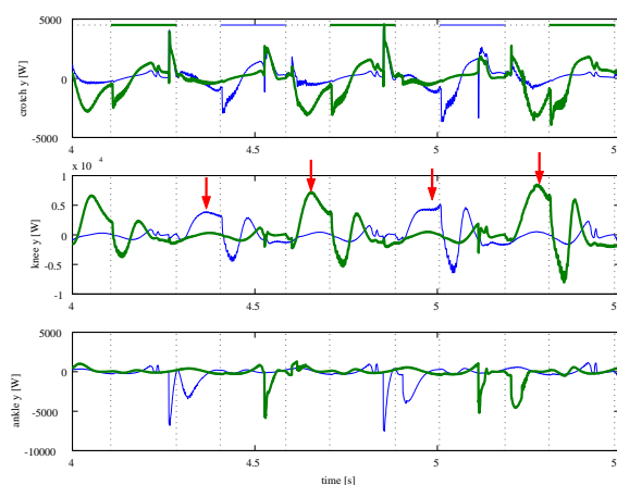
Figure 14: Joint power
