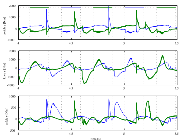
Figure 13: Joint torque
