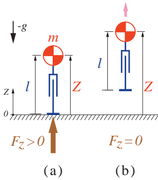
Figure 2: Take-off model
