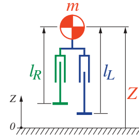
Figure 4: Biped model
