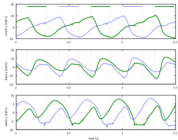
Figure 12: Joint speed
