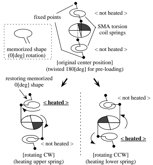
Fig. 4: Rotating actuator mechanism using SMA torsion coil springs.
