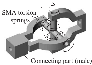
Fig. 10: Two-axis SMA actuator mechanism.
