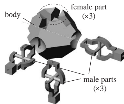
Fig. 11: A 3D module.
