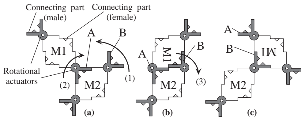
Fig. 1: Basic motion of two modules.
