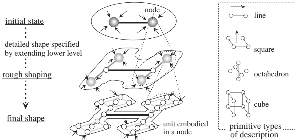
Fig. 14: Hierarchical graph structure for self-assembly.
