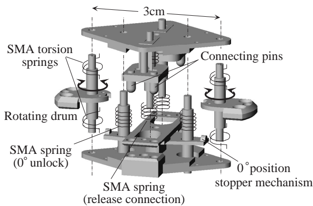
Fig. 4: Structure of micro-sized module.
