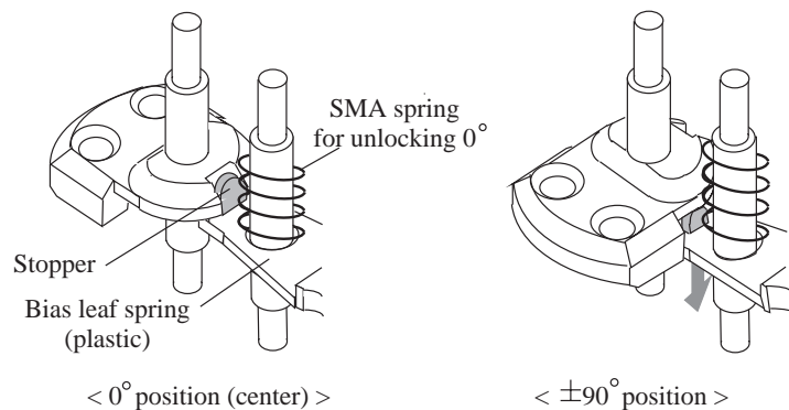
Fig. 6: Stopper mechanism of a male connecting part.
