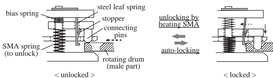
Fig. 7: Auto-locking mechanism of a female connecting part.
