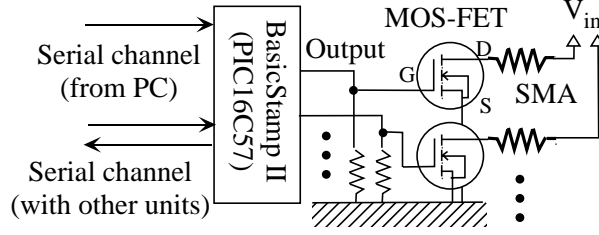
Fig. 8: Architecture of control unit.
