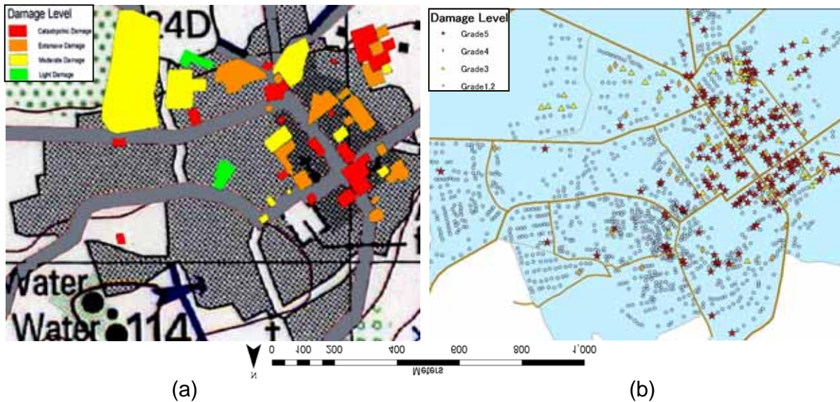
Figure 12. (a) Damage map for Zemmouri evaluated by the United States Government (UN-OCHA, 2003) and (b) our detection result
