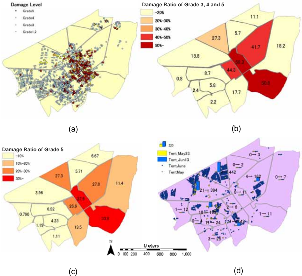
Figure 11. Building damage and tent distribution maps. (a) 1,399 buildings classified based on their damage grades, (b) the ratio of damaged buildings in each city block, (c) the ratio of Grade5 buildings in each city block, (d) the location of tents in the two post-event images
