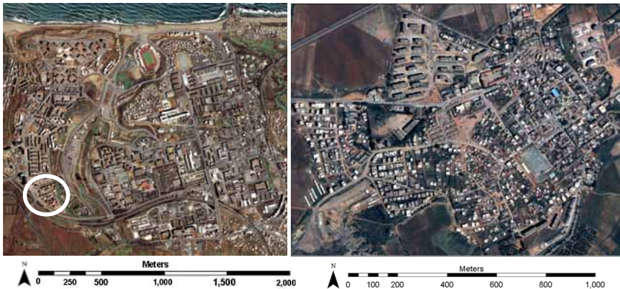
Figure 2. Pan-sharpened natural color QuickBird images acquired on May 23, 2003 (left: Boumerdes, right: Zemmouri).
