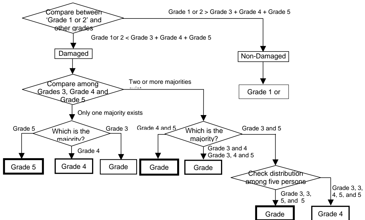
Figure 8. Flowchart to decide the majority damage level from the results by the five interpreters
