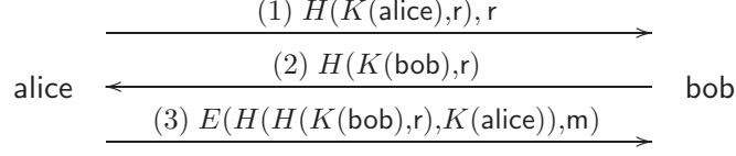
Fig. 8. Diffie-Hellman key-exchange algorithm
