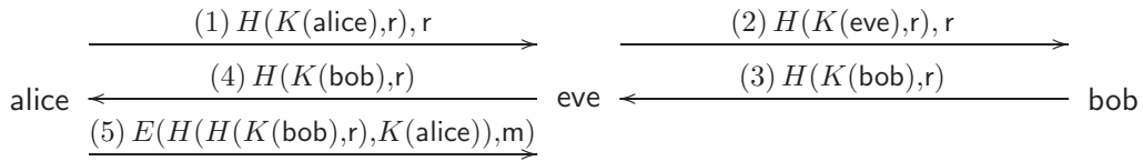
Fig. 10. Man-in-the-middle attack in Diffie-Hellman key exchange protocol
