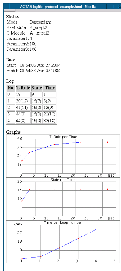
Fig. 7. Tool support for state space analysis
