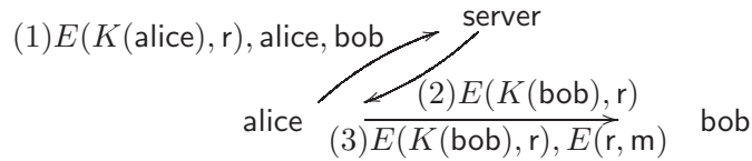
Fig. 3. A cryptographic protocol
