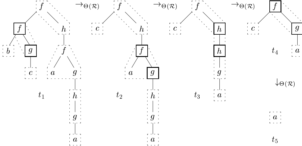
Figure 2: The maximal well-typed parts along a rewrite sequence.
