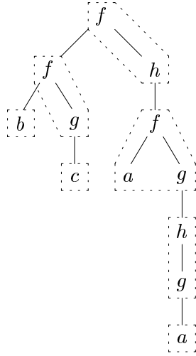
Figure 1: The maximal well-typed parts of t_1 .
