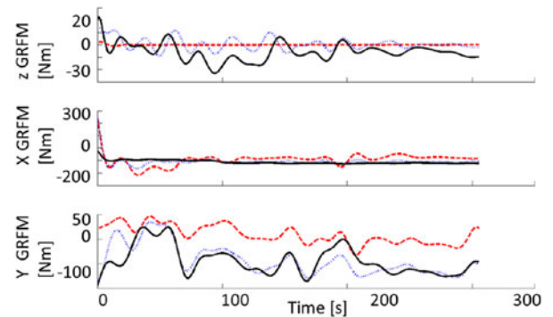
Fig. 9. GRFMs in vertical and horizontal directions reconstructed using identified BSIPs (blue dotted line) and BSIPs from the Dumas database (red dashed line), obtained using force plates measurements (black solid line).
